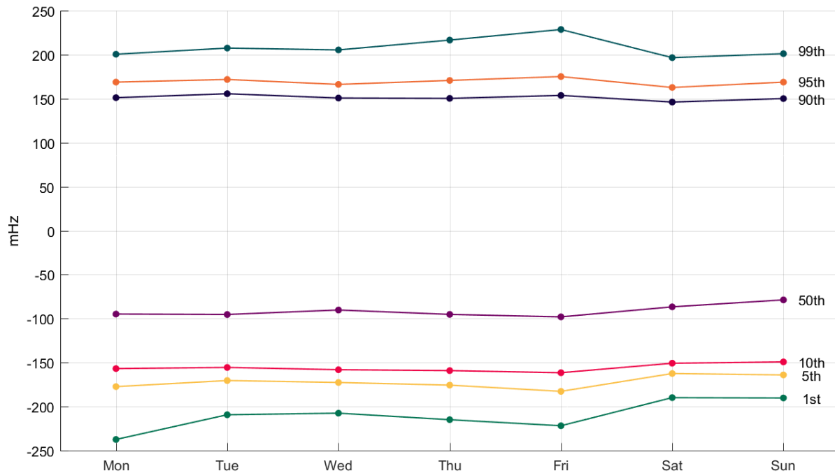
Figure 3.71. The 1st, 5th, 10th, 50th, 90th, 95th, and 99th percentile of deterministic frequency deviation for every day of the week in 2016
