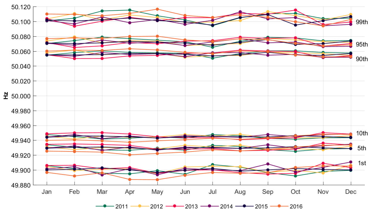
Figure 3.16. The 1st, 5th, 10th, 90th, 95th and 99th percentiles for years 2011-2016
