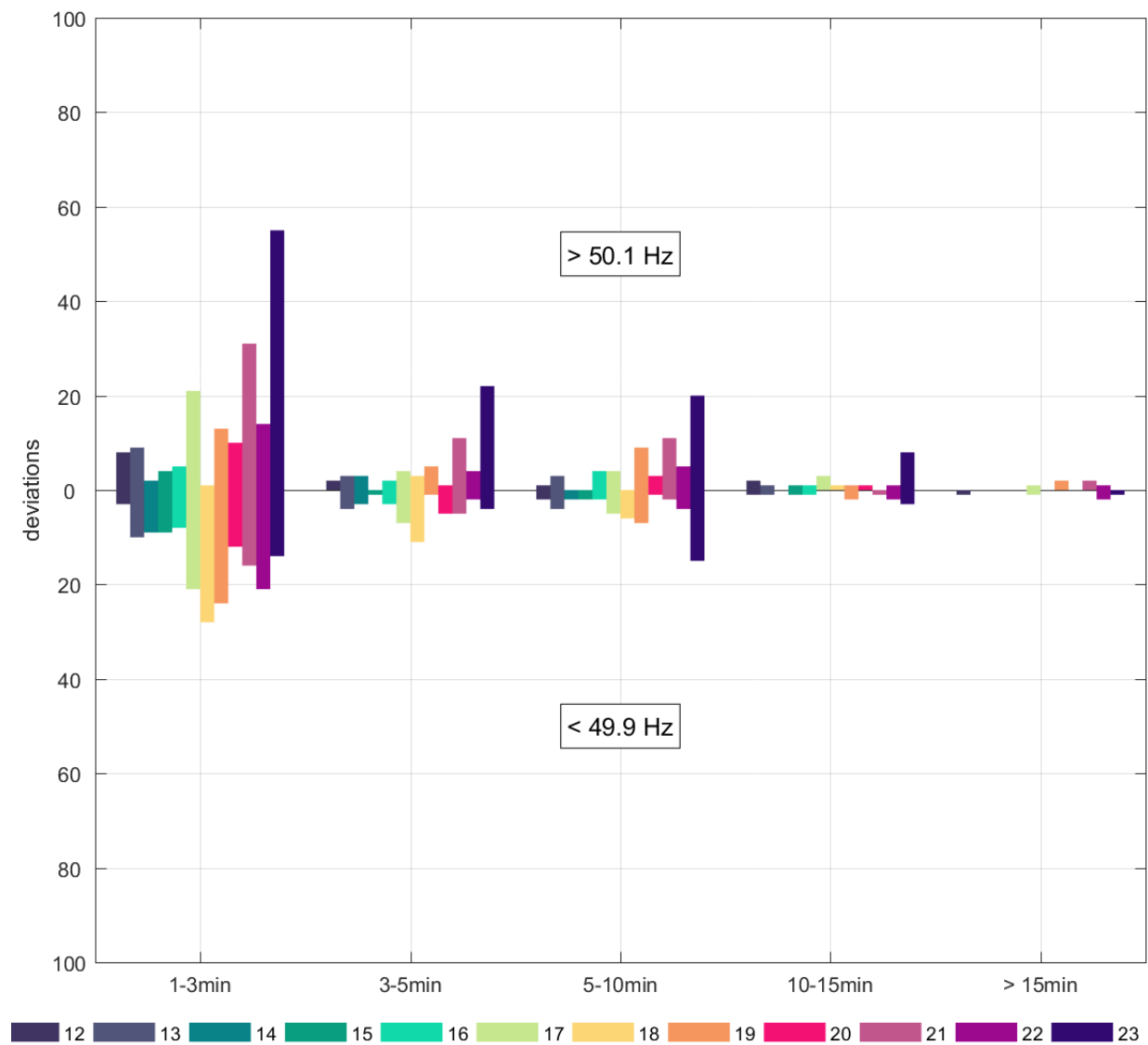
Figure 3.44. Total number of longer frequency deviations per duration for hours 12-23 in 2016
