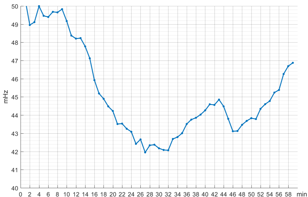
Figure 3.8. Standard deviation of the frequency for every minute of the hour in 2016
