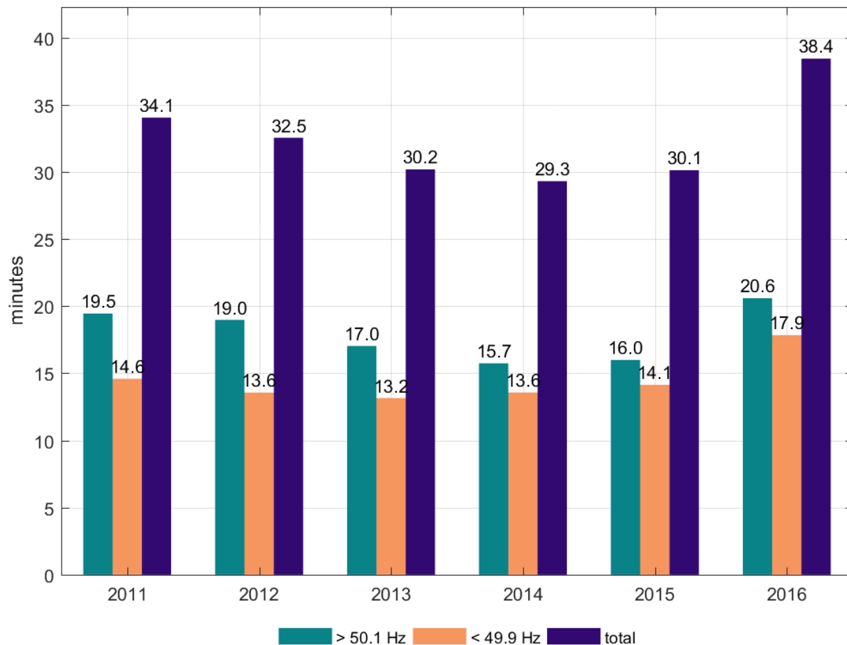
Figure 3.23. Daily average number of minutes per year that the frequency was outside the standard frequency range in 2011-2016
