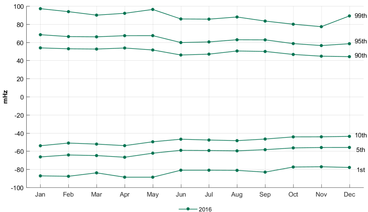
Figure 3.21. The 1st, 5th, 10th, 90th, 95th and 99th percentiles for year 2016
