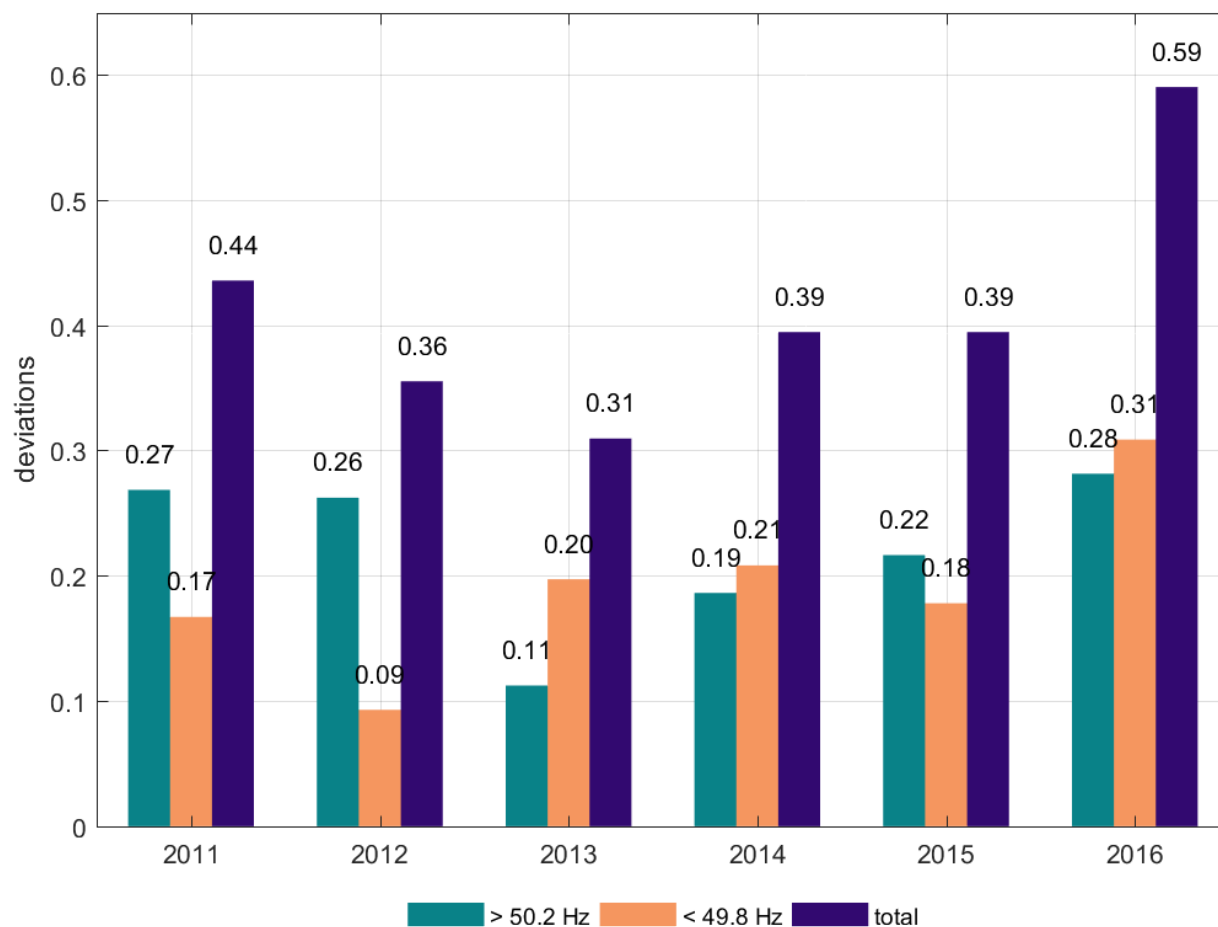
Figure 3.50. Daily average number of frequency deviations larger than \pm 200 mHz for years 2008-2016
