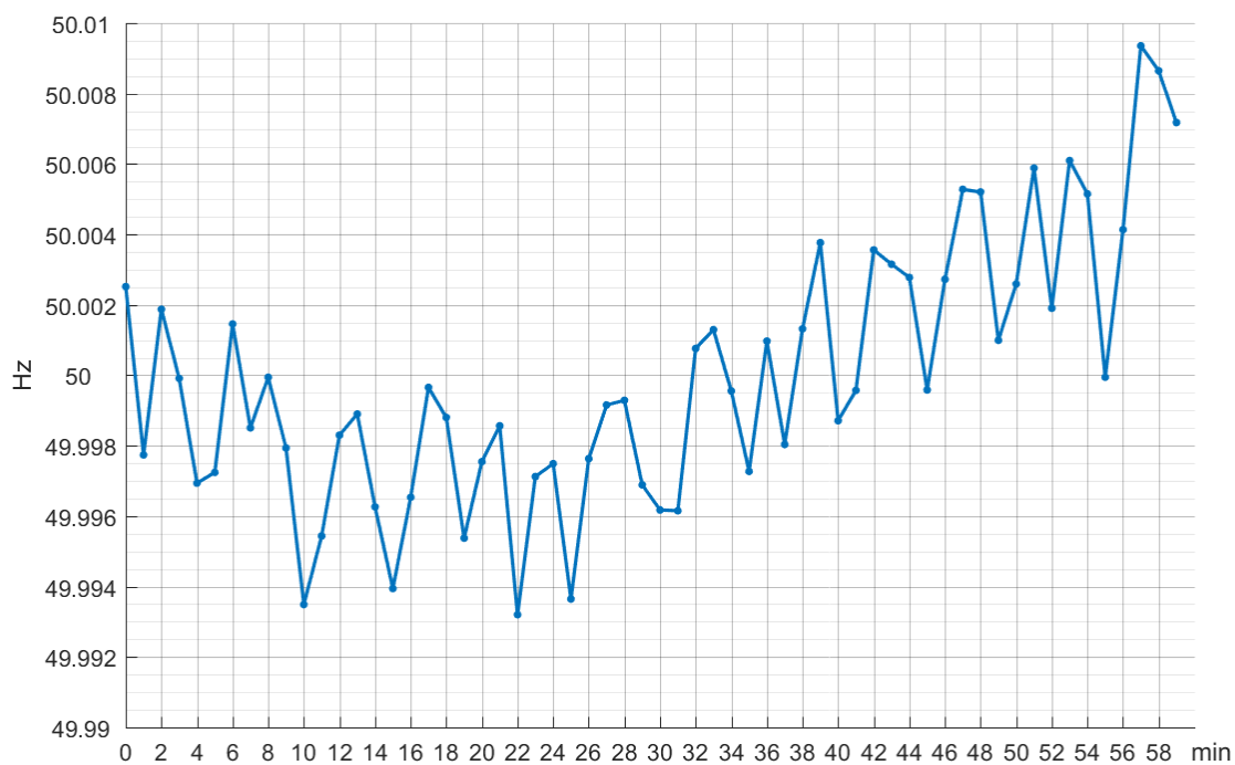
Figure 3.4. Average frequency for each minute of the hour in 2016
