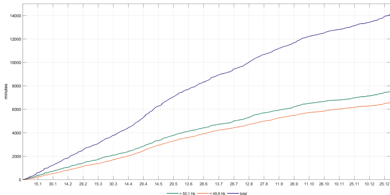
Figure 3.22. Cumulative minutes outside the standard frequency range in 2016
