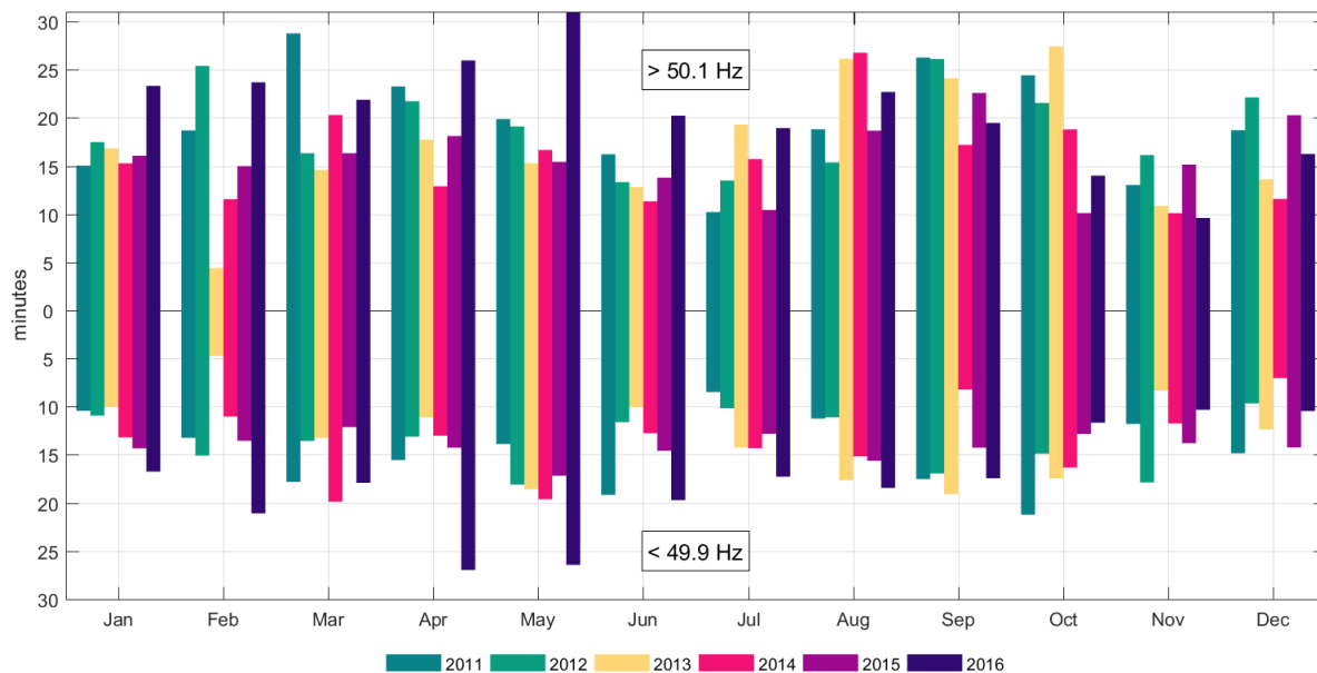
Figure 3.25. Daily average time that the frequency was outside the standard frequency range month by month for years 2011-2016
