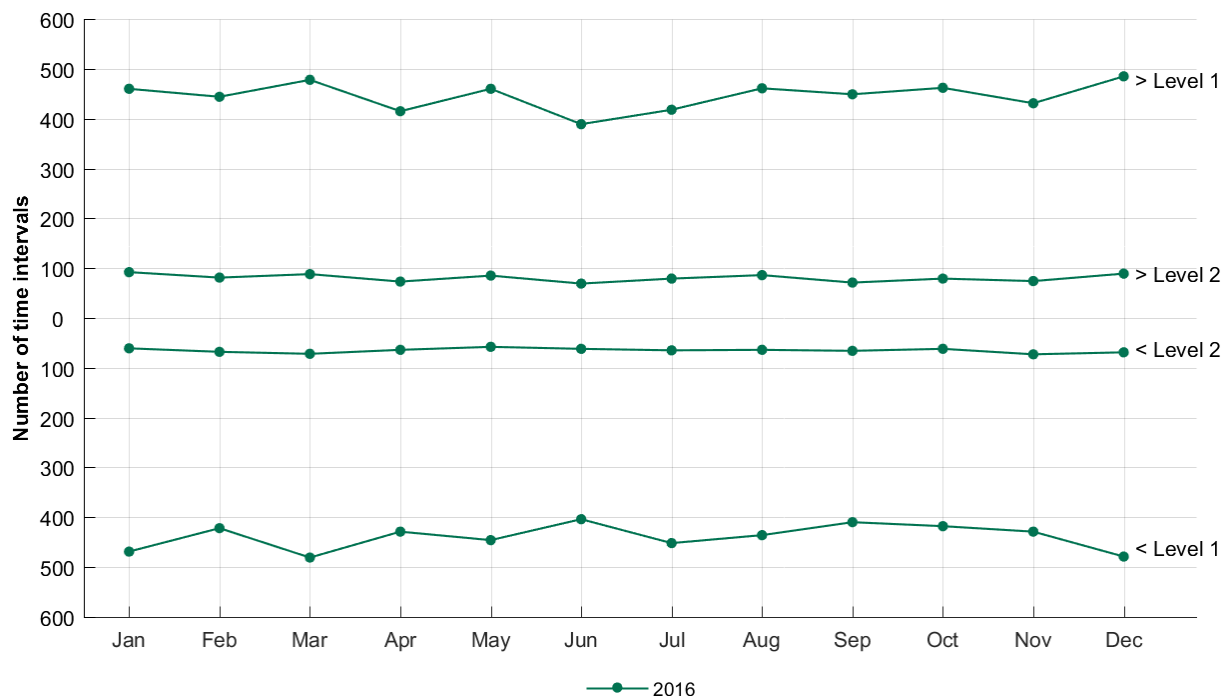
Figure 3.68. The number of time intervals over positive and under negative FRCE Level 1 and Level 2 Ranges for year 2016
