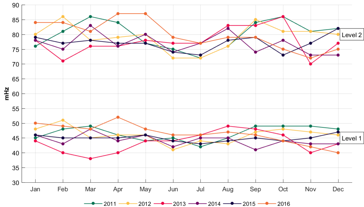
Figure 3.67. FRCE Ranges for years 2011-2016 calculated with 15 min moving averages
