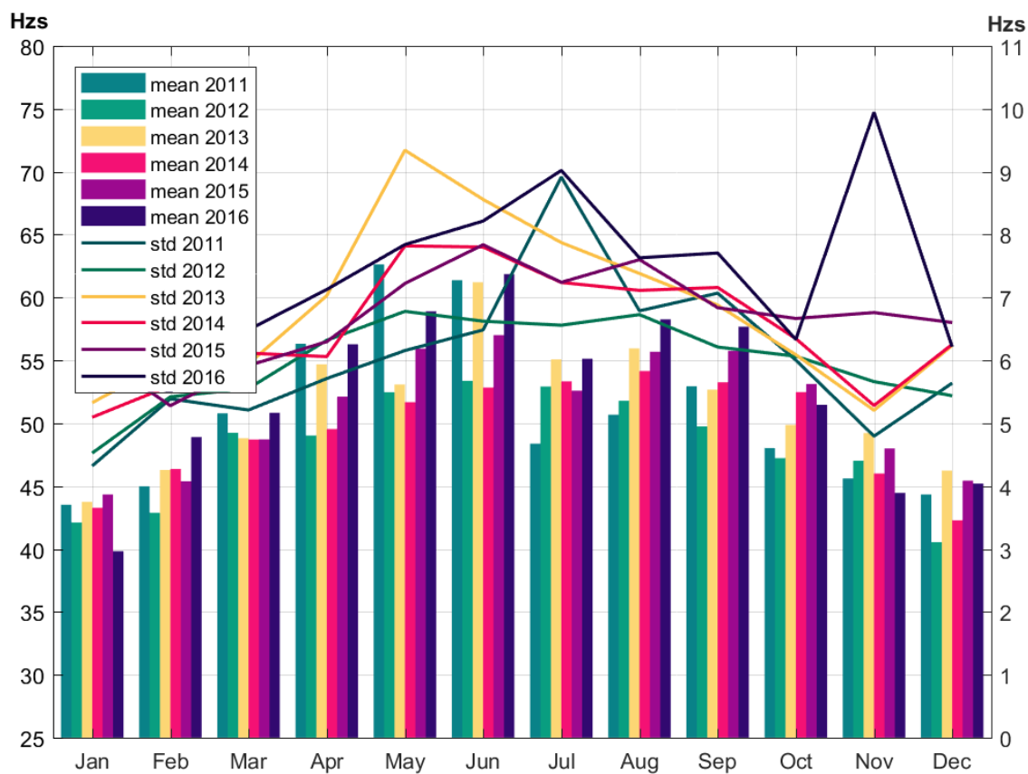
Figure 3.62. Mean values (left y-axis) and standard deviations (right y-axis) for oscillation in years 2011-2016
