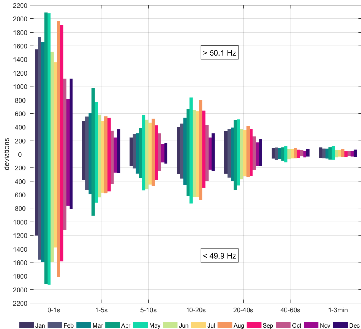
Figure 3.36. Total number of frequency deviations per duration for each month in 2016
