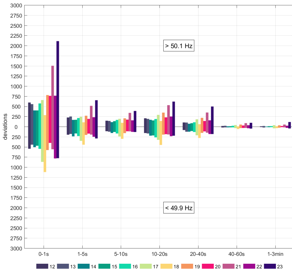
Figure 3.39. Total number of frequency deviations per duration for hours 12-23 in 2016
