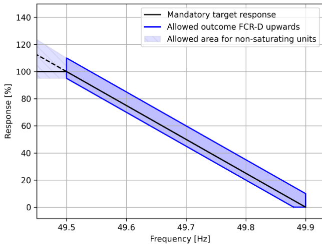
Figure 15. Activation of piecewise linear FCR-D resources. The black line indicates the mandatory target response. The controller shall be designed to minimise the deviation from the target response. The blue area defines the allowed outcome of the deviations, due to e.g. non-linear effects or step sizes for relay connected loads. The coordinates of the corners are provided in Table 9 below.
