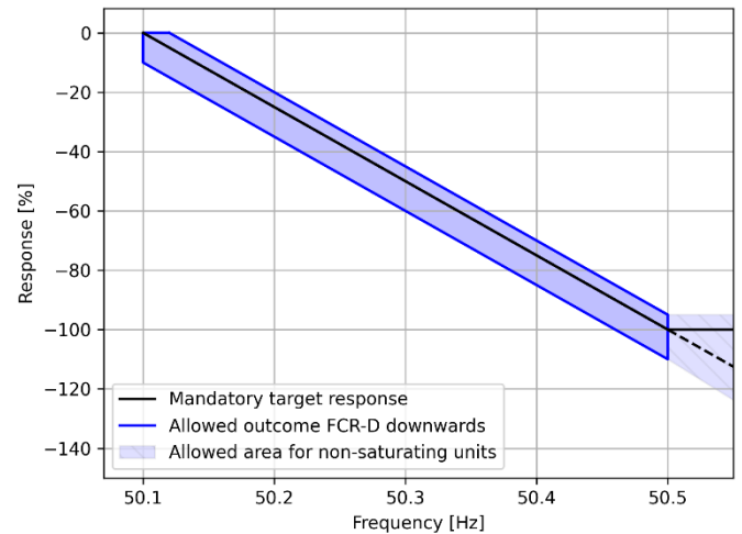
Figure 15. Activation of piecewise linear FCR-D resources. The black line indicates the mandatory target response. The controller shall be designed to minimise the deviation from the target response. The blue area defines the allowed outcome of the deviations, due to e.g. non-linear effects or step sizes for relay connected loads. The coordinates of the corners are provided in Table 9 below.
