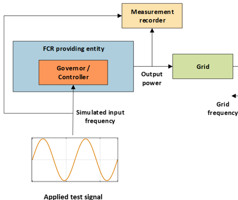
Figure 29. Test setup.
