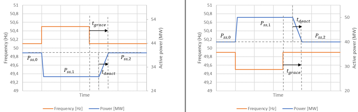
Figure 6. Illustration of a Static FCR-D ramp test and the notation used in the requirements.
